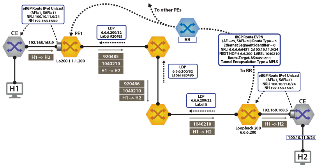
Figure 121: Control Plane & Forwarding Tenant-A Over LDP
