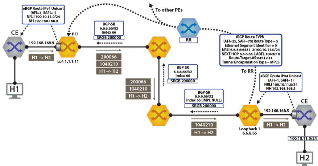
Figure 124: Control Plane & Forwarding Tenant-A Over BGP-SR
