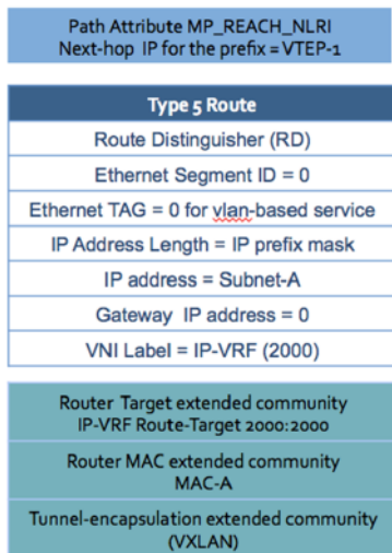
Figure 109: EVPN Type-5 Route Format for Interface-less Mode
