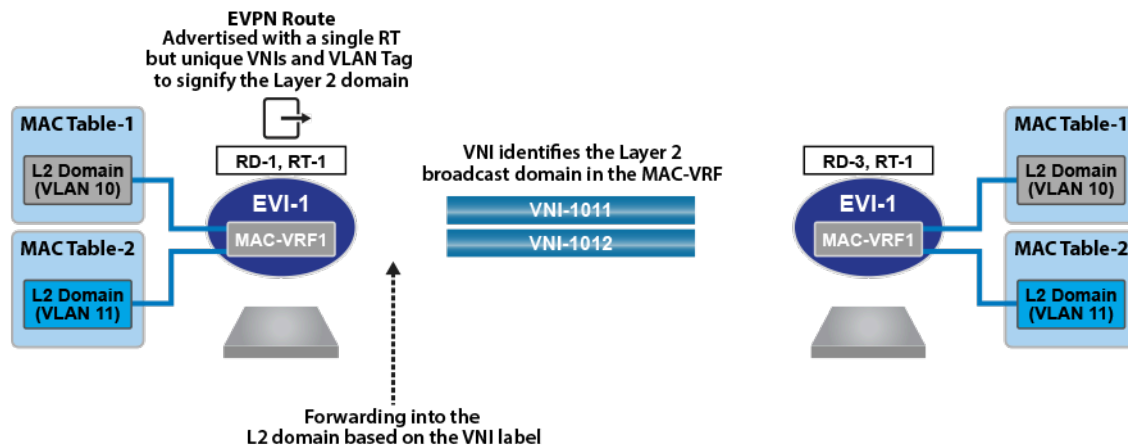
Figure 76: VLAN Aware Bundle Service
