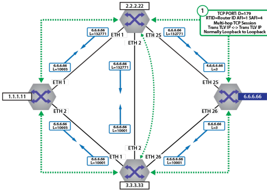
Figure 105: BGP-LU Label Distribution
