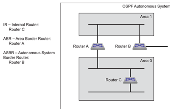
Figure 43: OSPFv2 Router Types
