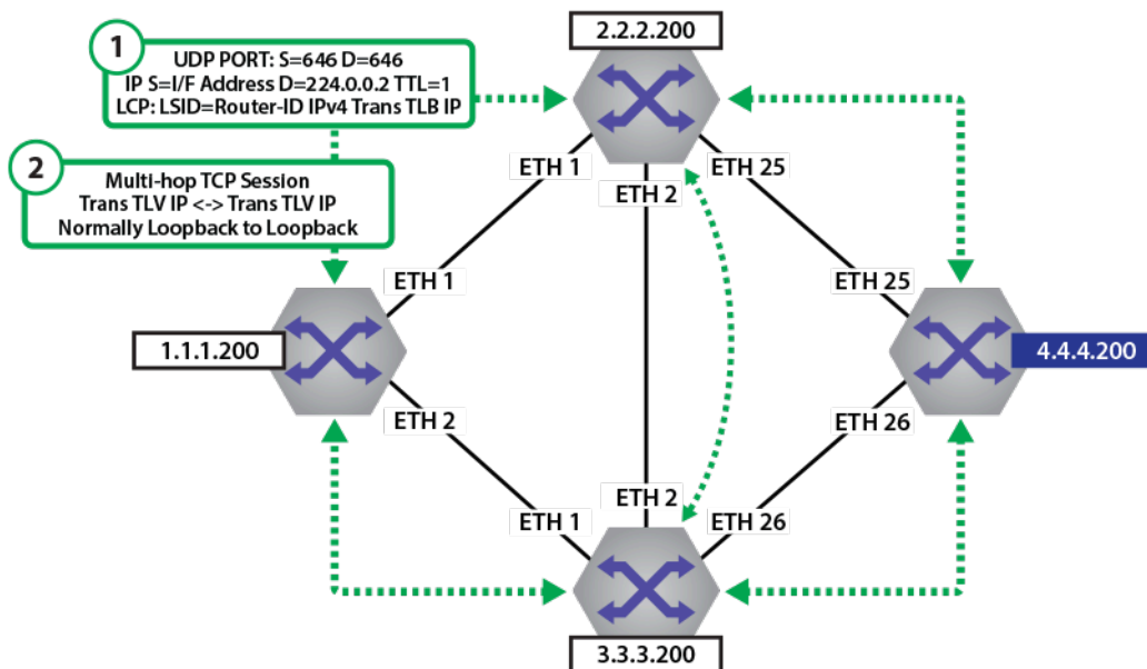
Figure 103: LDP Peering Establishment
