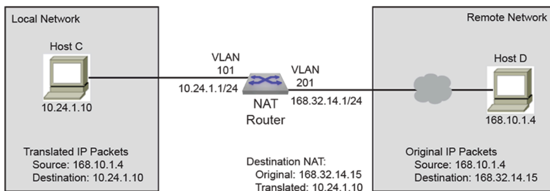
Figure 9: Detination NAT Example
