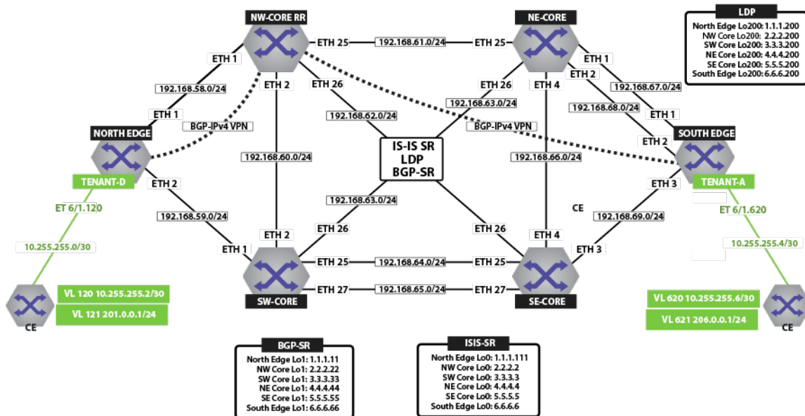
Figure 125: IPv4 VPN Physical Topology
