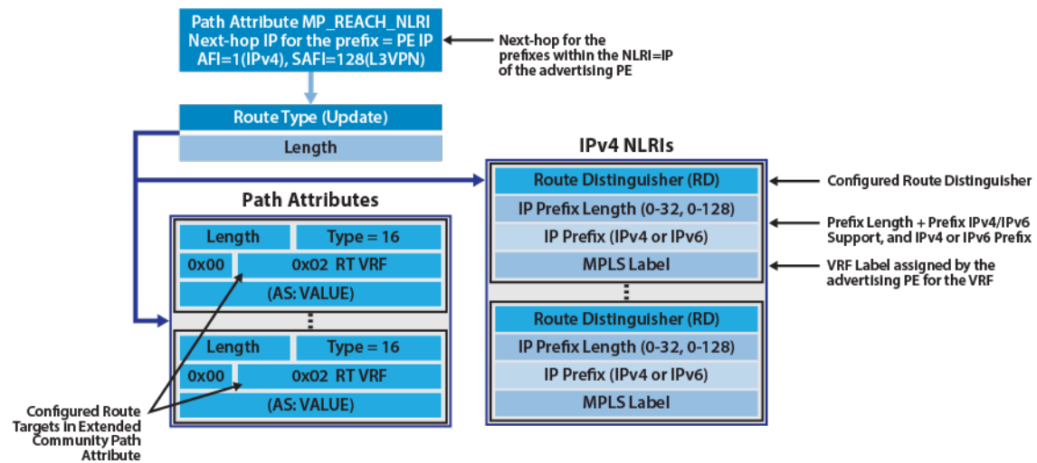
Figure 93: IPv4 and IPv6 VPN Update Route Detail
