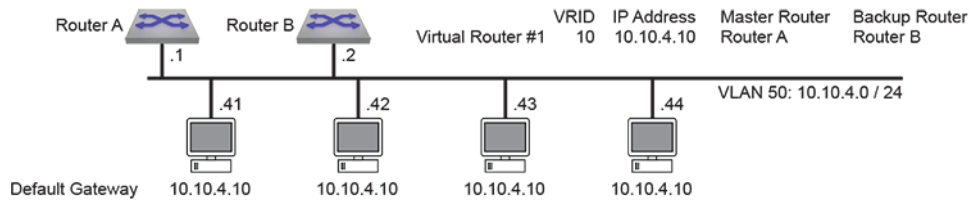
Figure 30: VRRP Example 1 Network Diagram
