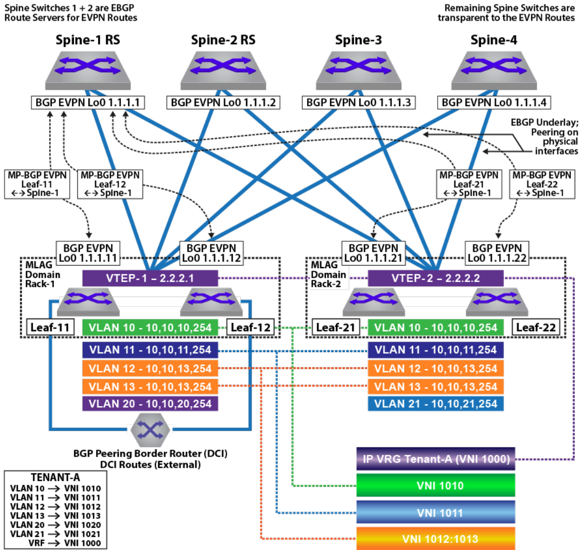
Figure 113: Tenant-A: Symmetric IRB
