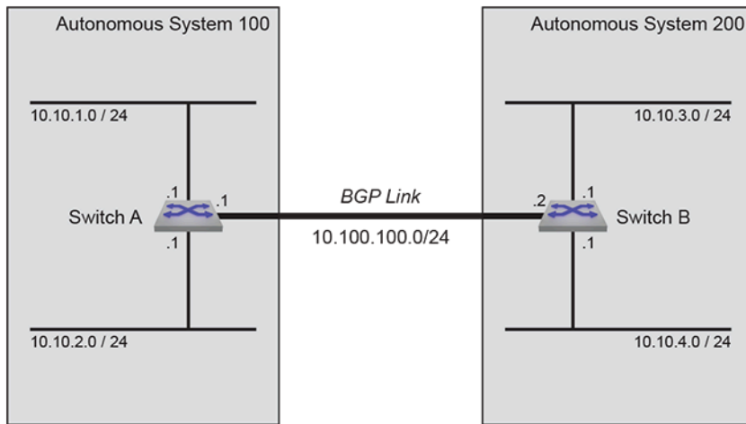
Figure 58: BGP Example 2
