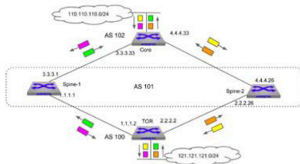
Figure 59: Traffic flow pattern between TOR and Core Before Maintenance
