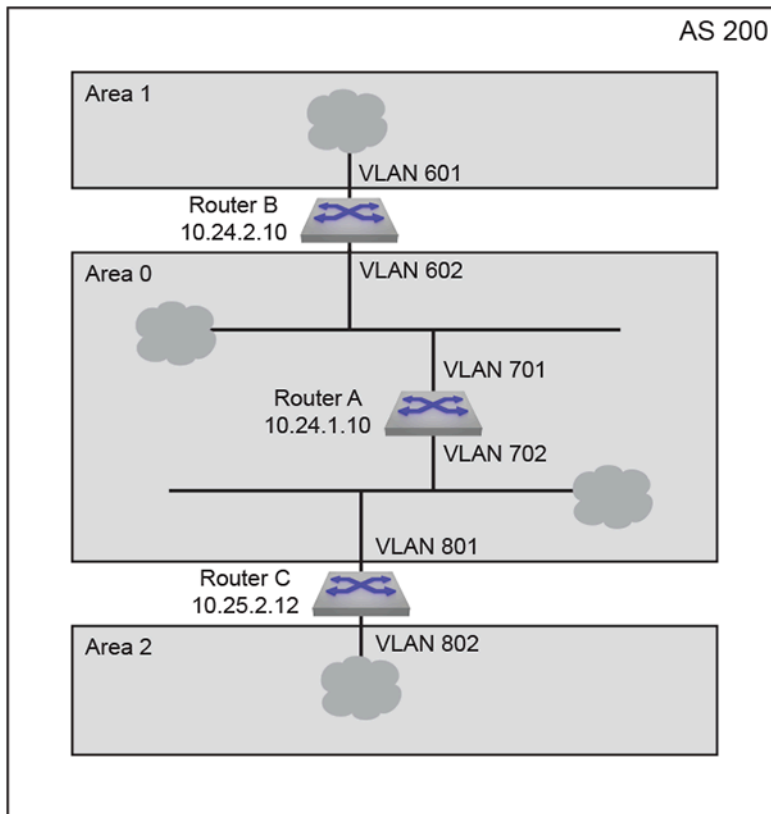
Figure 51: OSPFv3 Example 2
