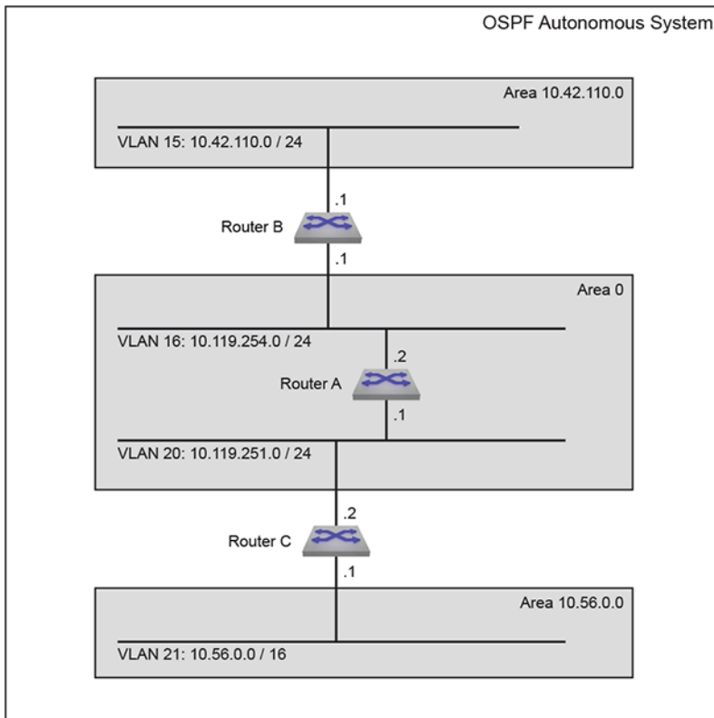
Figure 46: OSPFv2 Example 2
