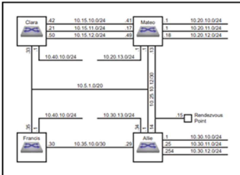
Figure 64: Multicast Example
