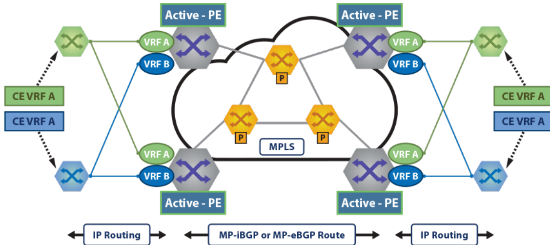
Figure 96: MPLS Layer 3 VPN Topology
