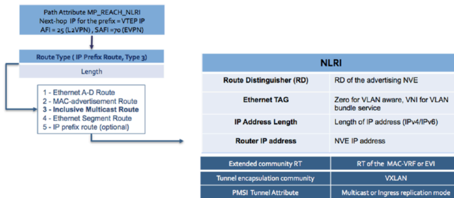
Figure 84: EVPN Type-3 IMET Route Format
