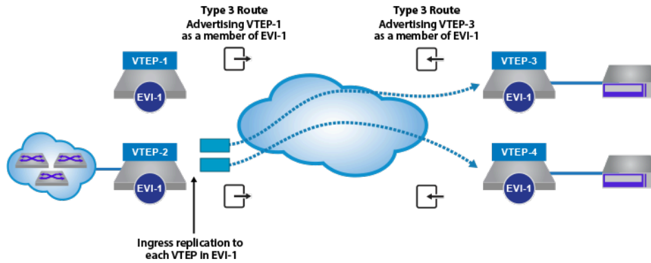
Figure 83: EVPN type-3 IMET Route Behavior for Ingress Replication
