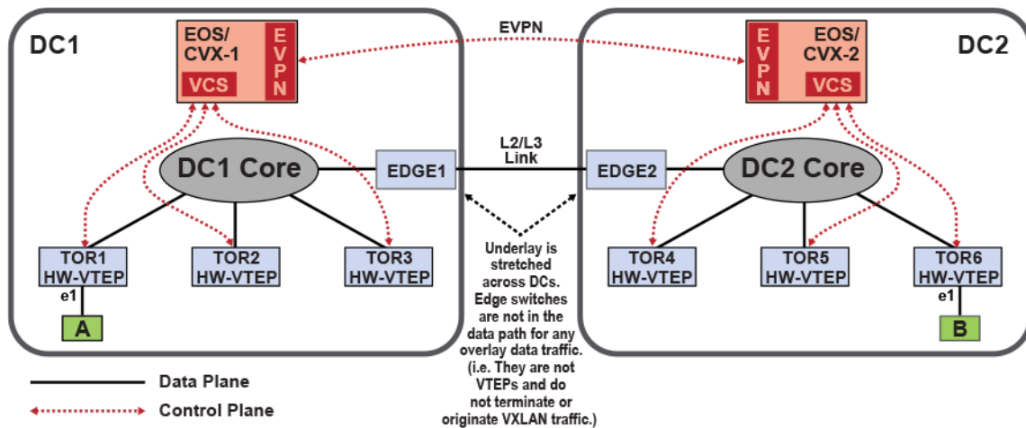
Figure 77: CVX Connected from Multiple DCs
