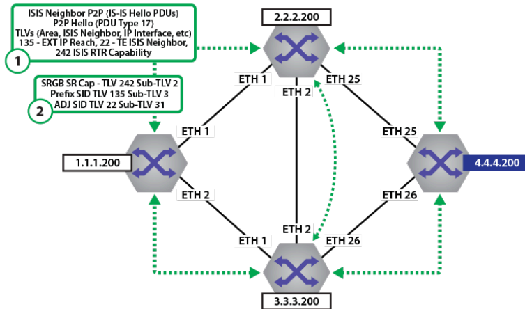
Figure 104: ISIS Neighbor Adj and TLVs
