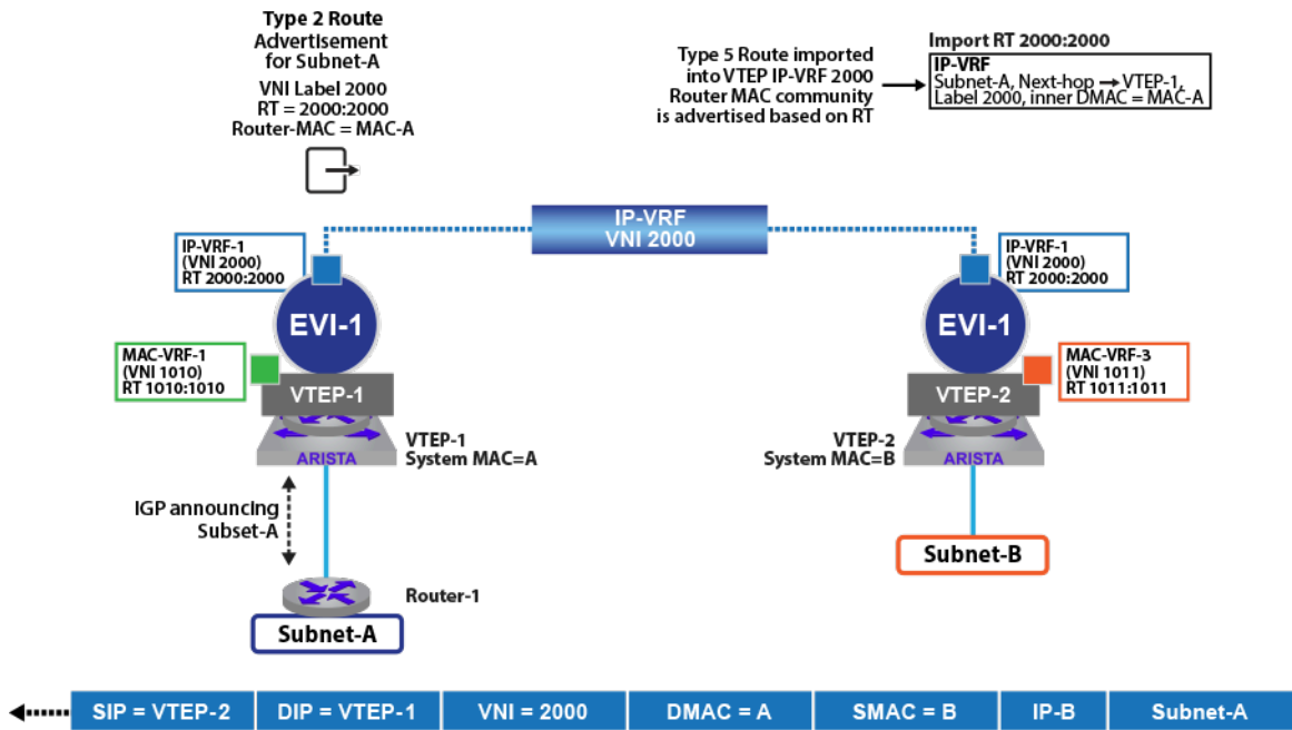
Figure 108: EVPN Route Type-5, Interface-less Update
