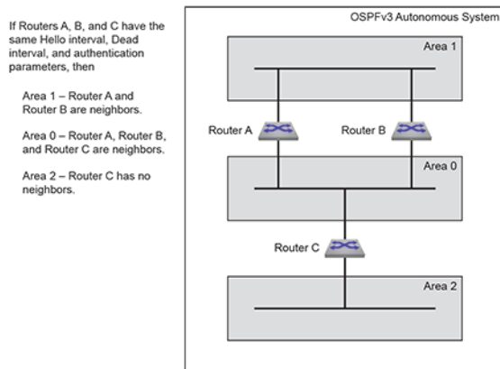
Figure 49: OSPFv3 Neighbors
