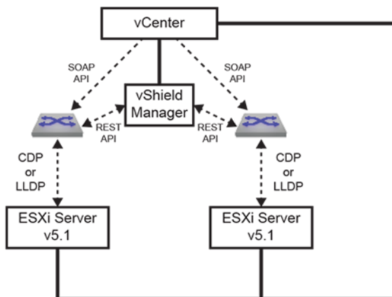
Figure 141: VM Tracer Topology – Monitoring VXLAN Based Configurations
