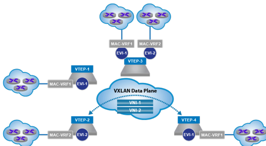
Figure 71: EVPN Terminology for a VXLAN Data Plane
