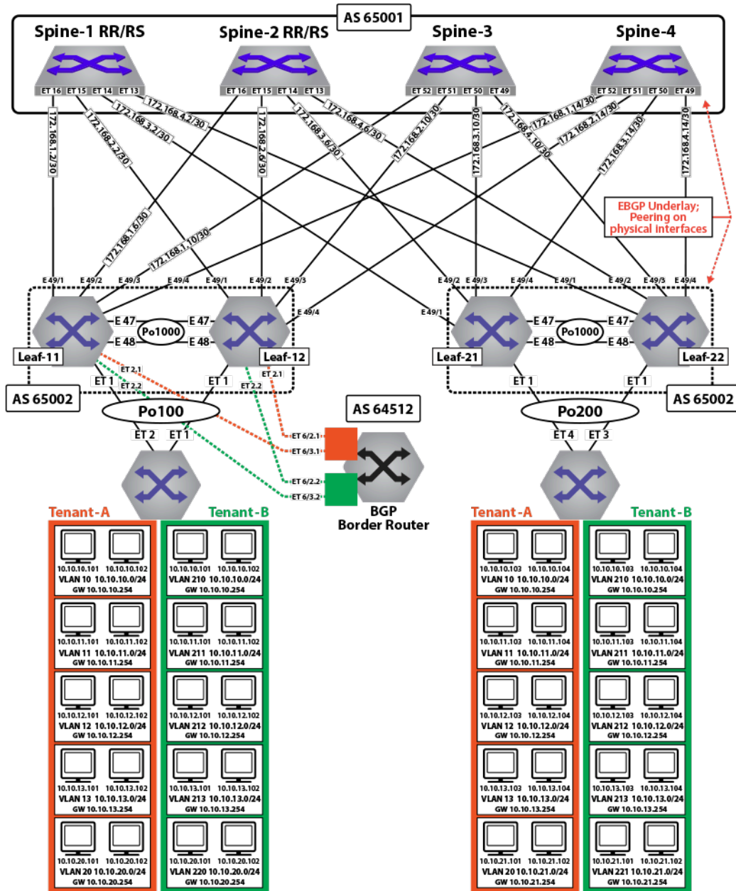
Figure 115: Physical Underlay Topology
