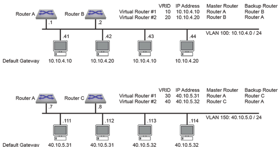
Figure 32: VRRP Example 3 Network Diagram
