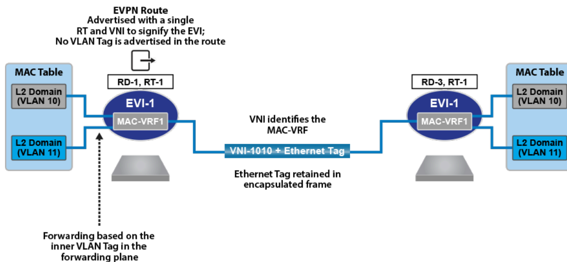
Figure 75: VLAN Bundle Service Interface
