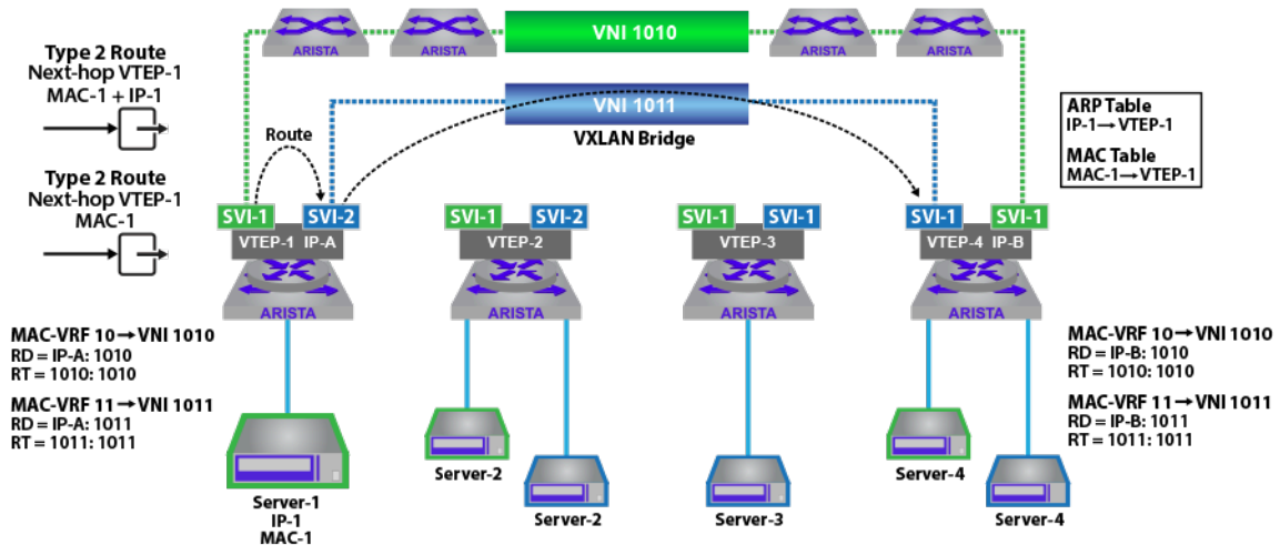
Figure 85: EVPN Asymmetric IRB
