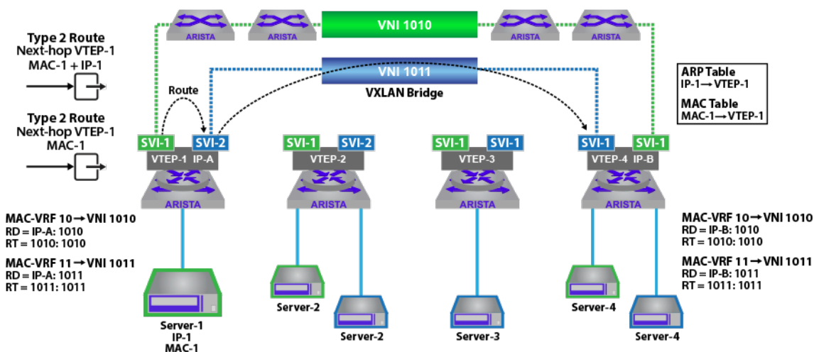
Figure 88: EVPN Symmetric IRB
