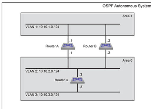
Figure 45: OSPFv2 Example 1
