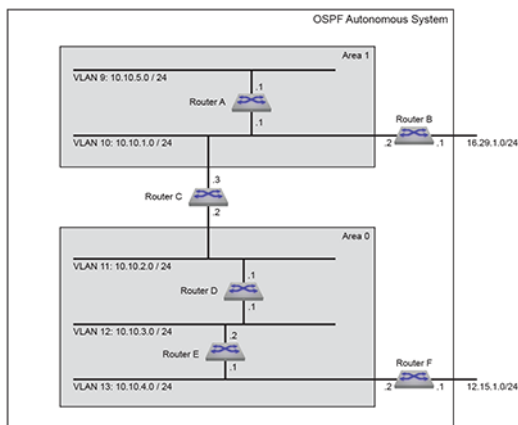
Figure 47: OSPFv2 Example 3
