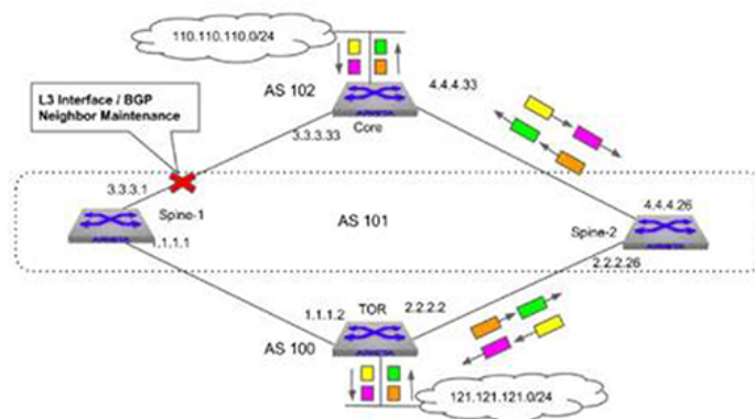
Figure 60: Traffic flow pattern between TOR and Core After unit on Spine-1 is put into Maintenance
