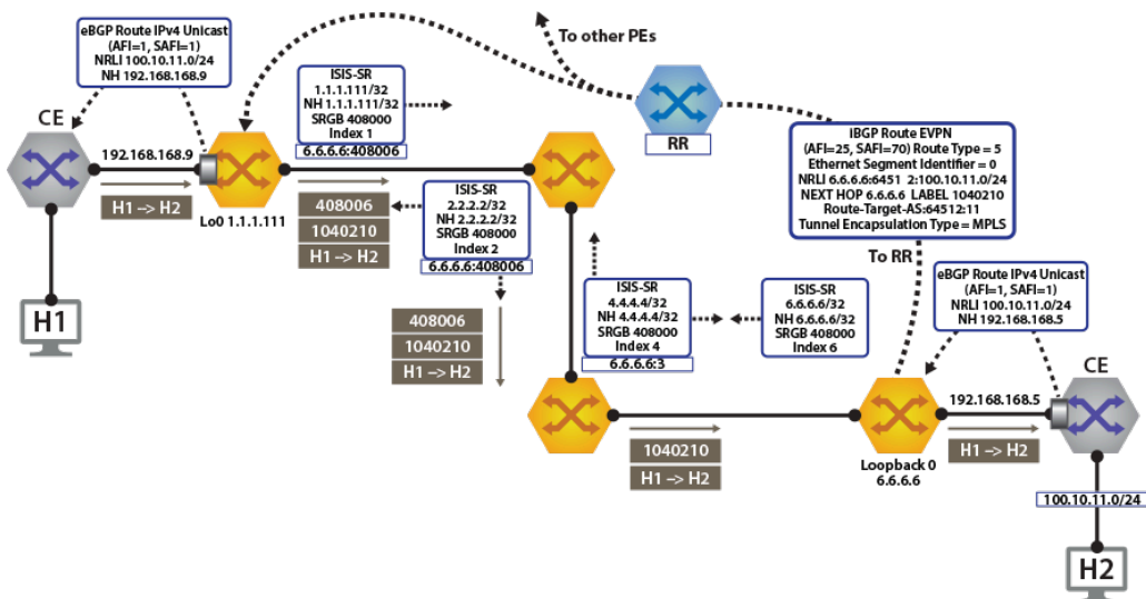
Figure 118: Control Plane & Forwarding Tenant-A Over ISIS-SR
