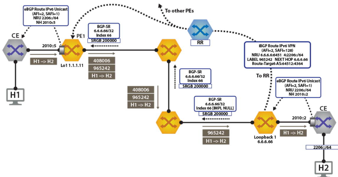
Figure 135: IPv6 VPN Forwarding Over BGP-SR MPLS
