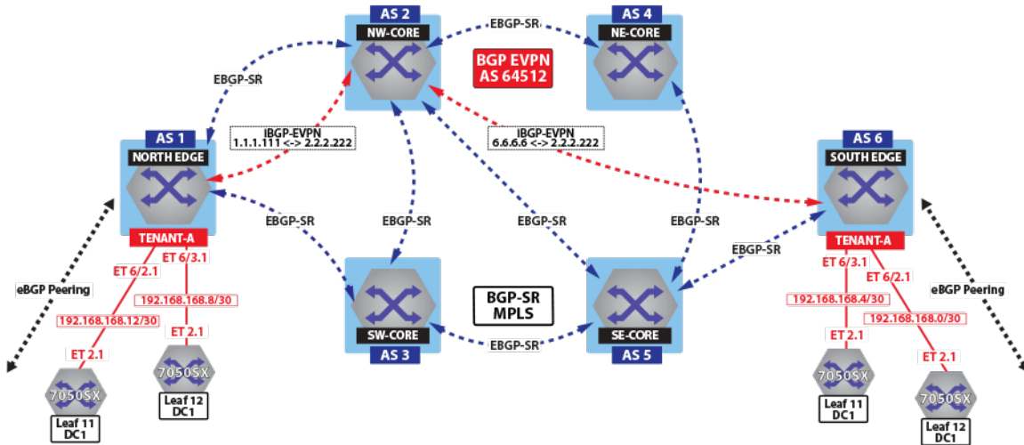
Figure 122: Control Plane Tenant-A Over BGP-SR
