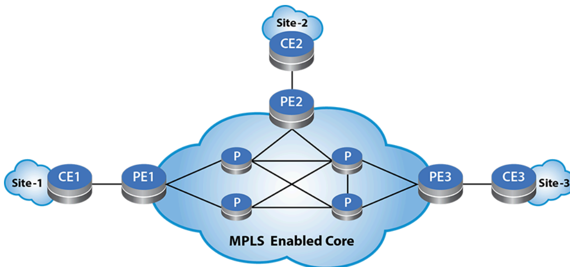
Figure 137: MPLS Enabled Core Schematic
