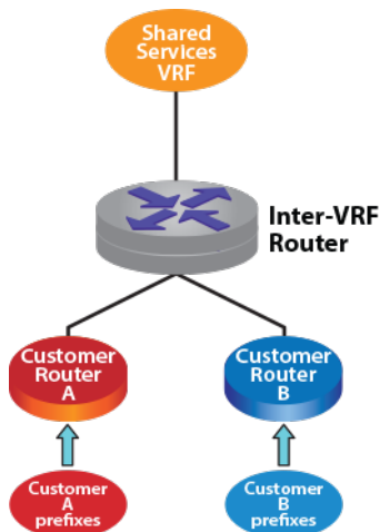
Figure 111: Accessing Shared Resources Across VPNs
