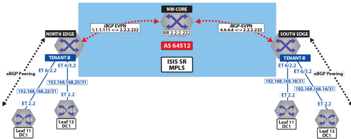
Figure 117: Control Plane Tenant-B over ISIS-SR
