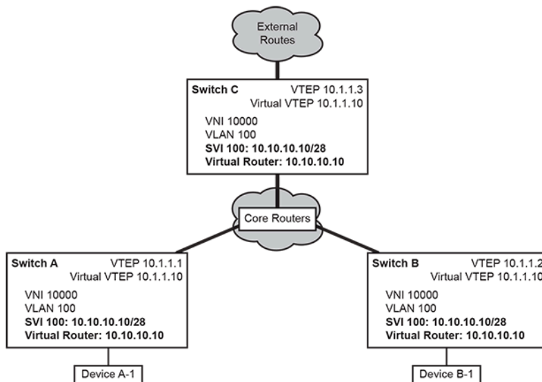
Figure 68: Direct VXLAN Routing
