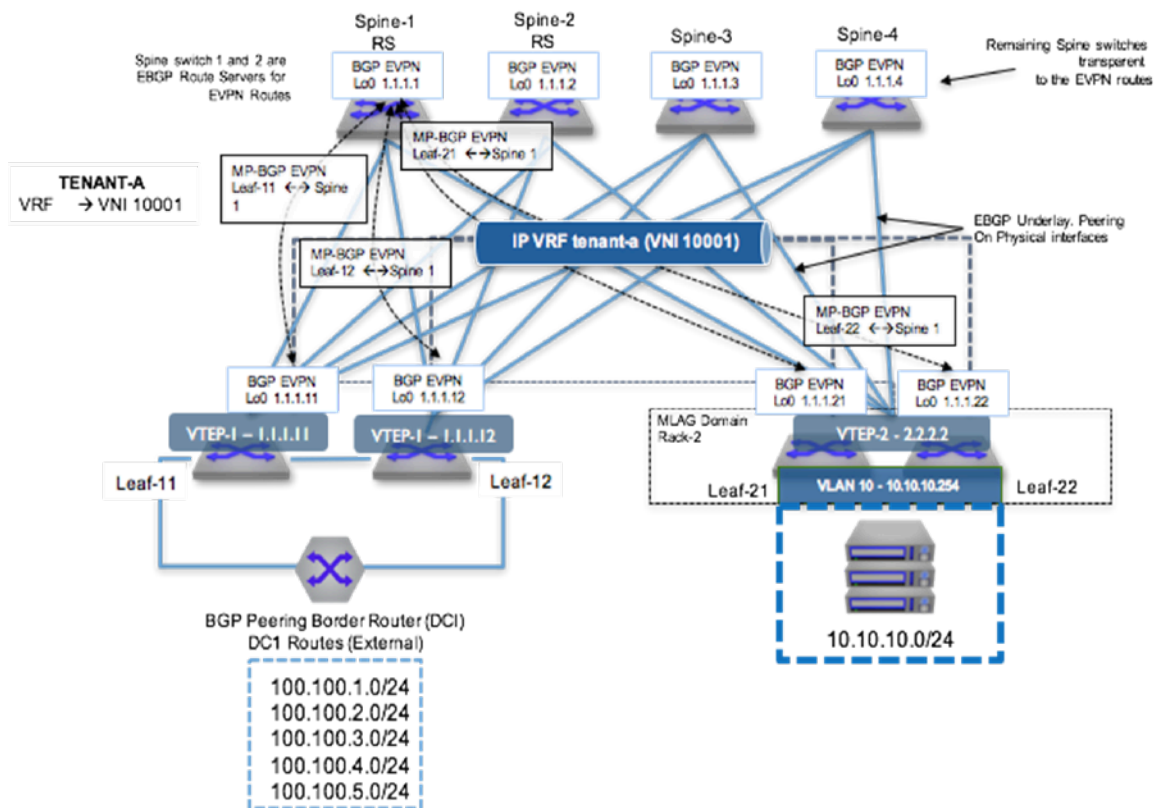
Figure 112: Layer 3 EVPN Configuration
