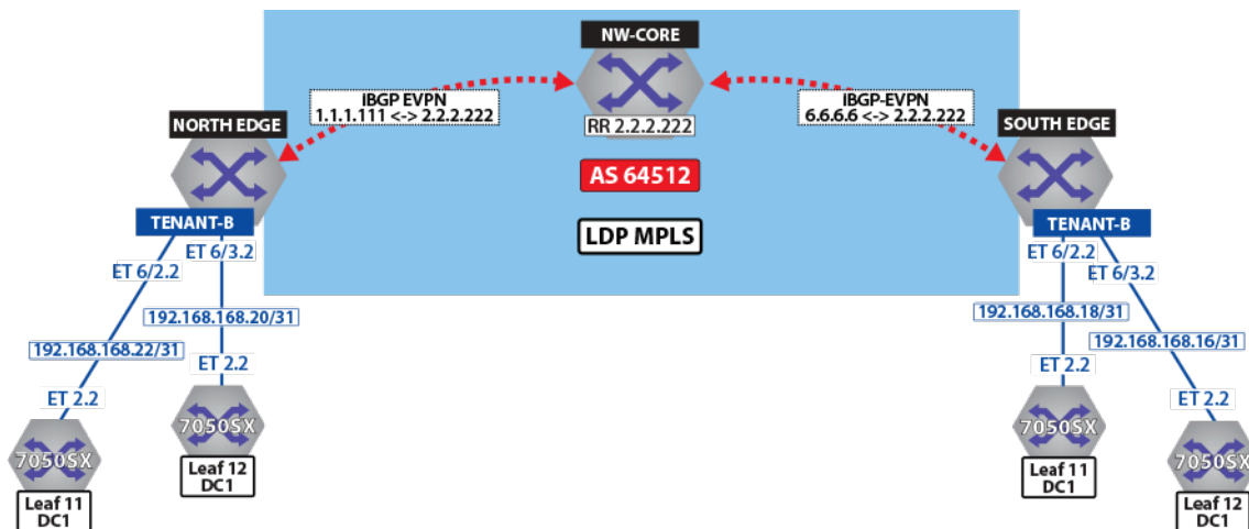
Figure 120: Control Plane Tenant-B over LDP
