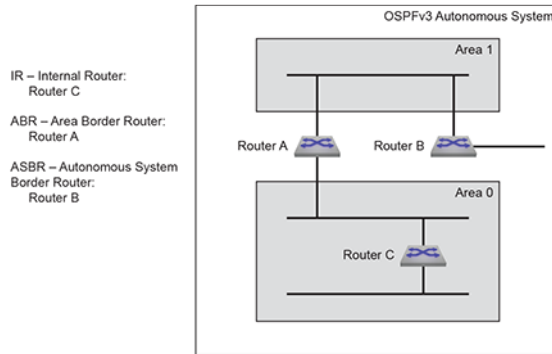
Figure 48: OSPFv3 Router Types
