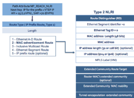
Figure 81: EVPN Type 2 MAC and IP Route Format
