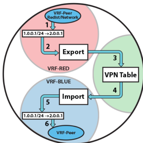
Figure 110: Inter-VRF Local Route Leaking using Local VPN Table
