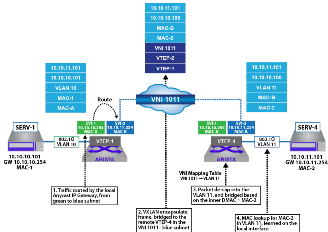
Figure 87: EVPN Asymmetric IRB VxLAN Data-plane Forwarding Detail
