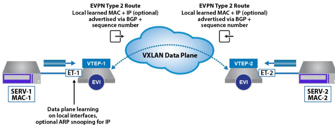
Figure 80: EVPN Type 2 Route Announcement
