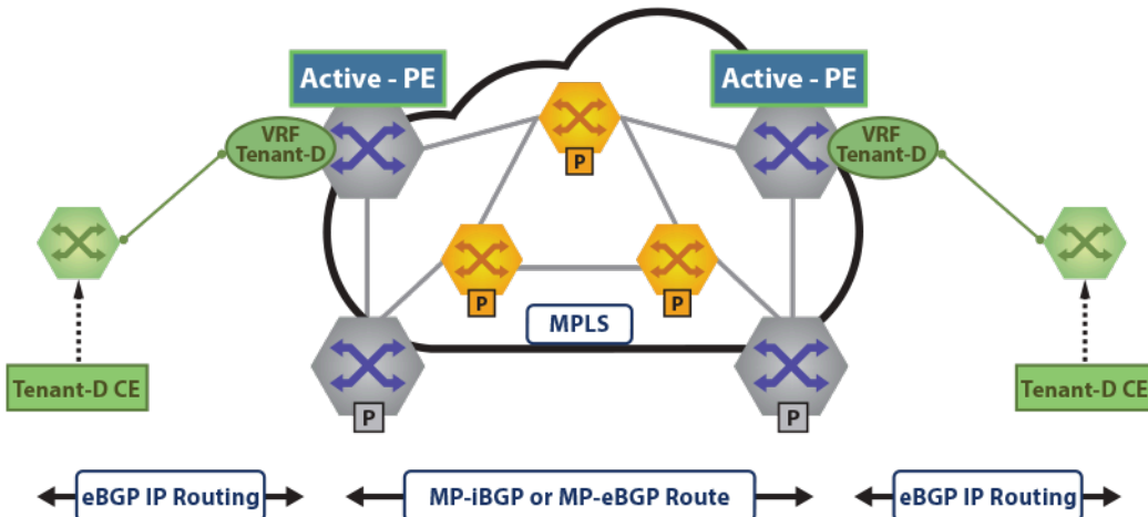
Figure 100: IPv4 & IPv6 VPN Sample Topology
