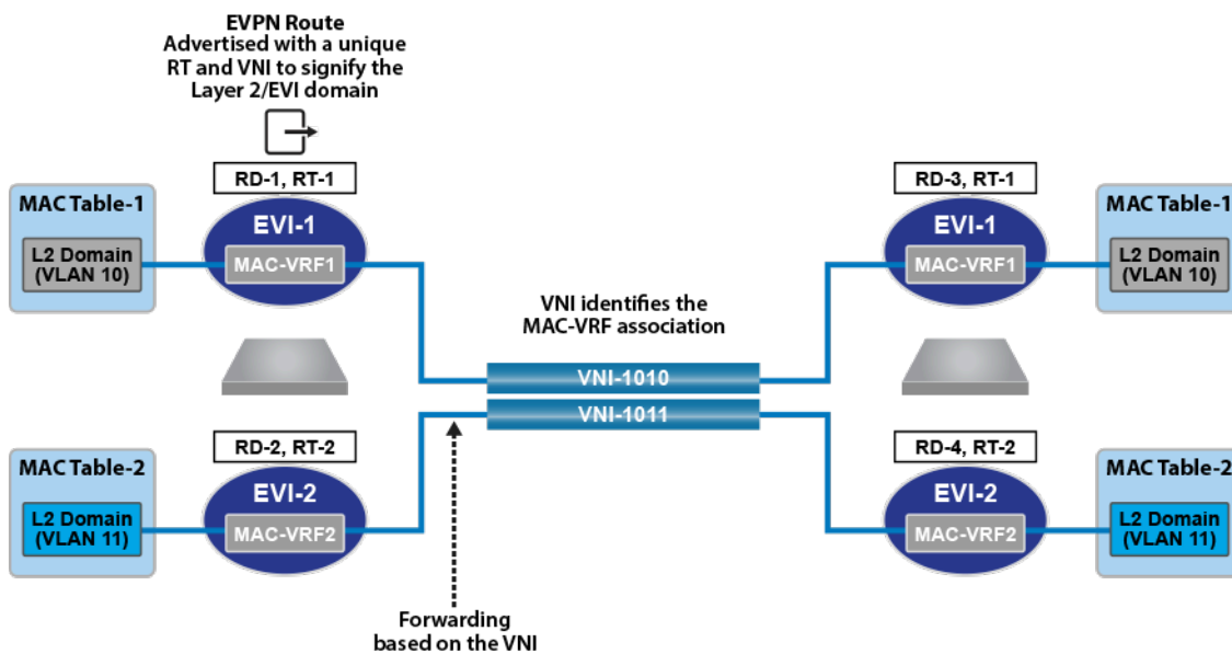
Figure 74: VLAN Based Service Interface
