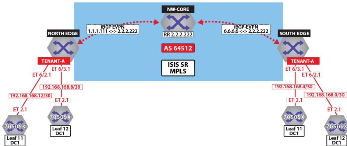
Figure 119: Control Plane Tenant-A Over LDP
