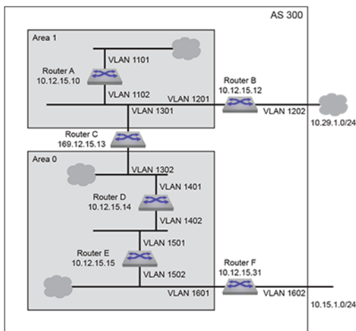
Figure 52: OSPFv3 Example 3
