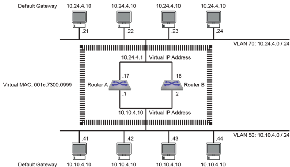
Figure 33: VARP Example Network Diagram
