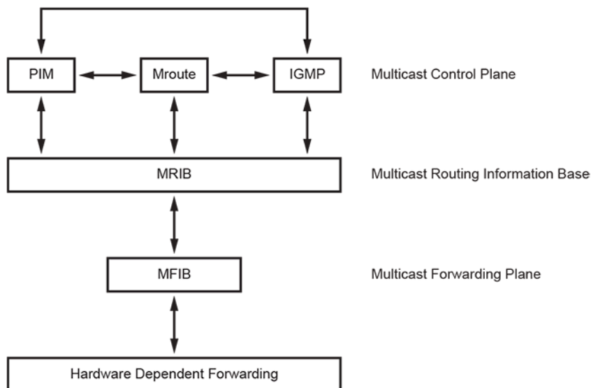
Figure 61: Multicast Architecture
