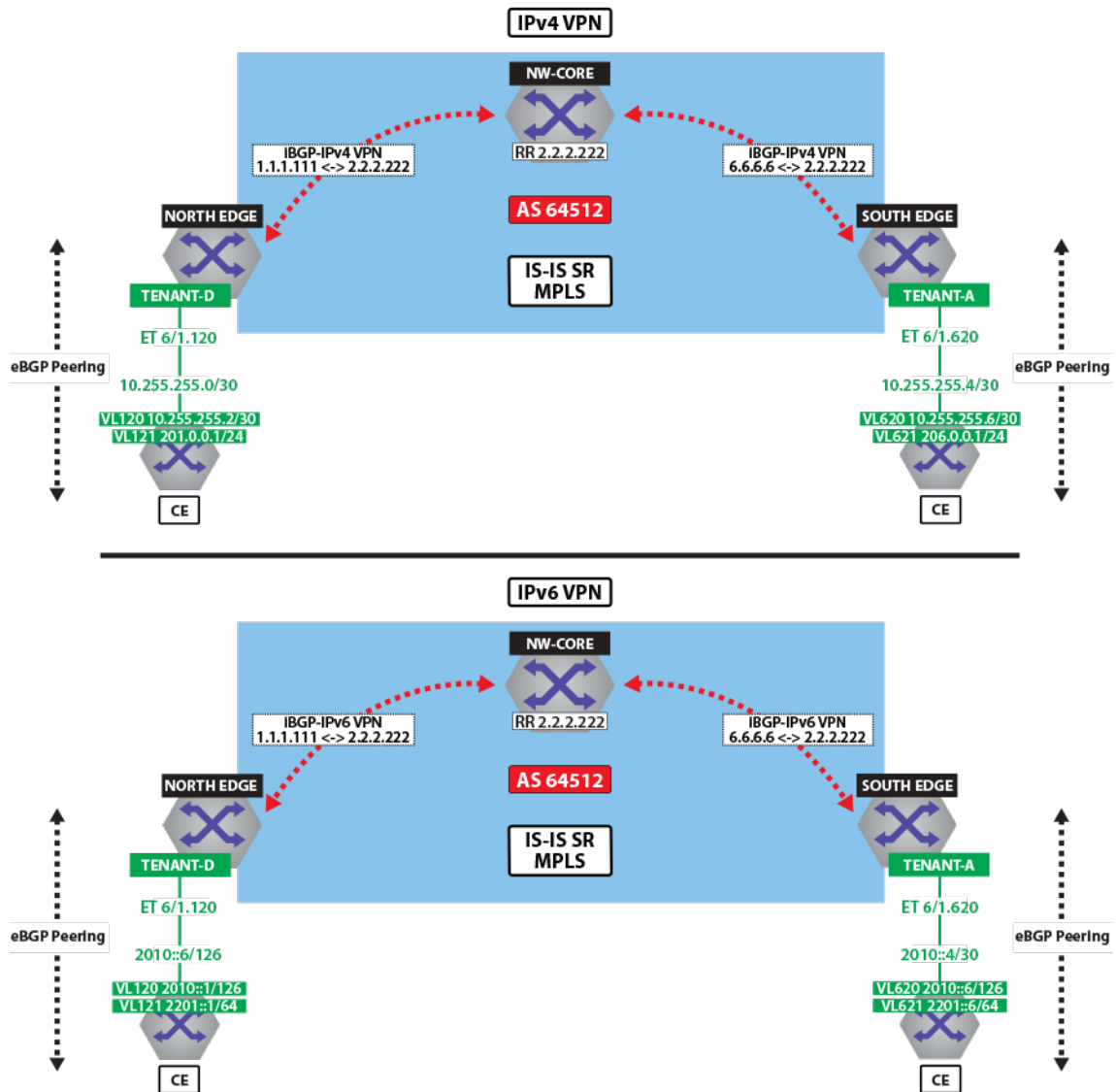
Figure 127: IPv4 VPN and IPv6 VPN Over IS-IS SR MPLS
