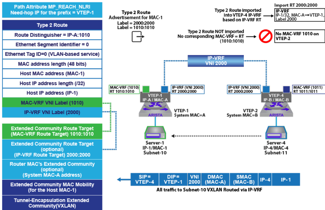
Figure 90: EVPN Type 2 Route in Symmetric IRB - MAC-VRF Only Exists on Sending VTEP
