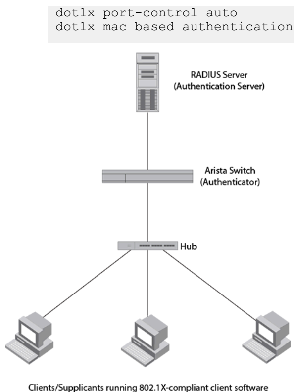
Figure 7: Multiple clients connected to a 802.1X-enabled port
