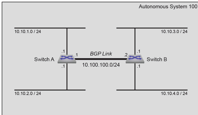
Figure 57: BGP Example 1
