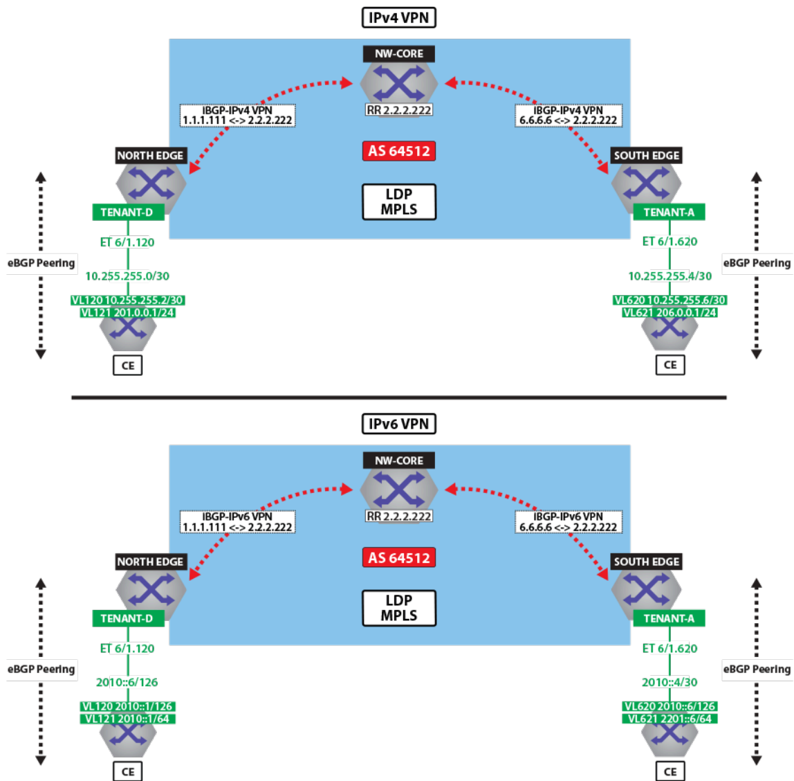
Figure 130: IPv4 VPN and IPv6 VPN Over LDP MPLS
