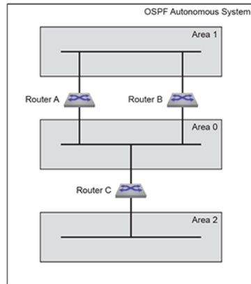
Figure 44: OSPFv2 Neighbors
