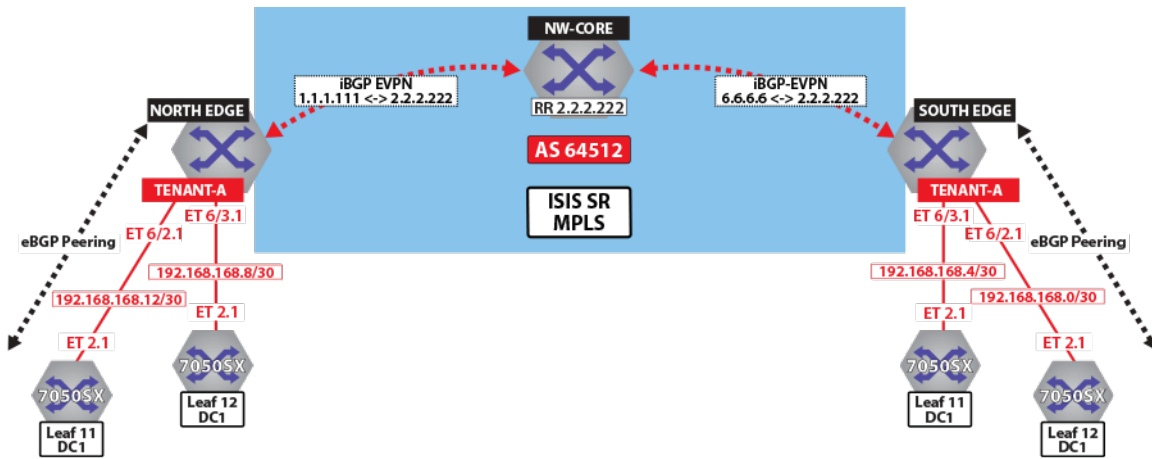
Figure 116: Control Plane Tenant-A Over ISIS-SR
