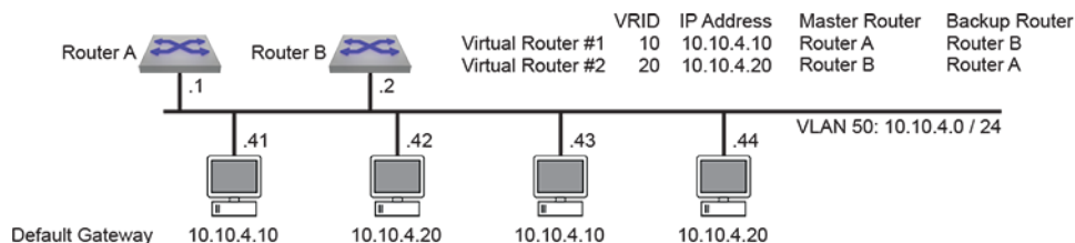
Figure 31: VRRP Example 2 Network Diagram
