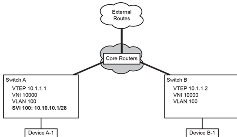
Figure 67: Implementing VXLAN Routing
