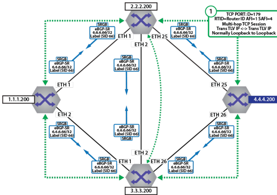
Figure 106: BGP-SR Index and SRGB Distribution
