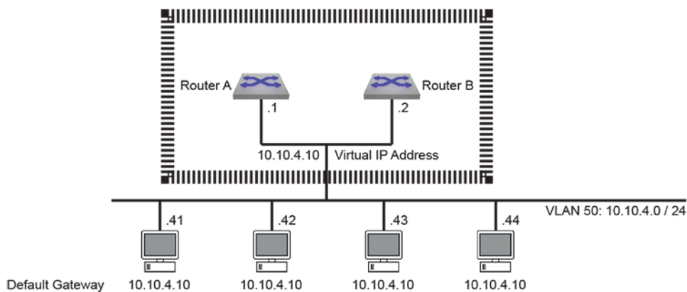
Figure 29: VARP Configuration
