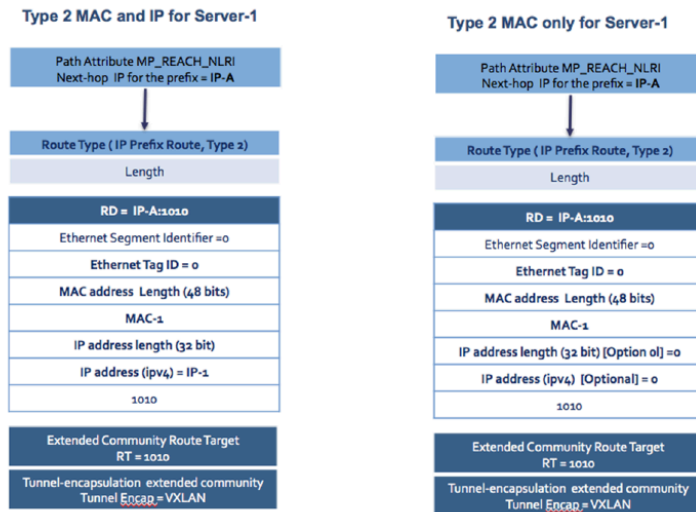
Figure 86: EVPN Comparison of MAC & MAC+IP Type 2 Route in Asymmetric IRB
