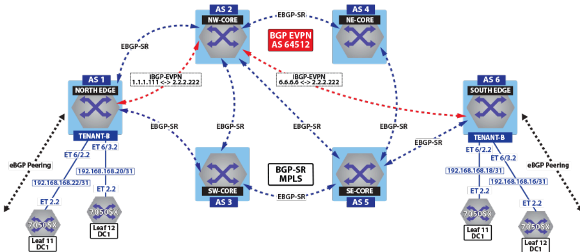
Figure 123: Control Plane Tenant-B Over BGP-SR
