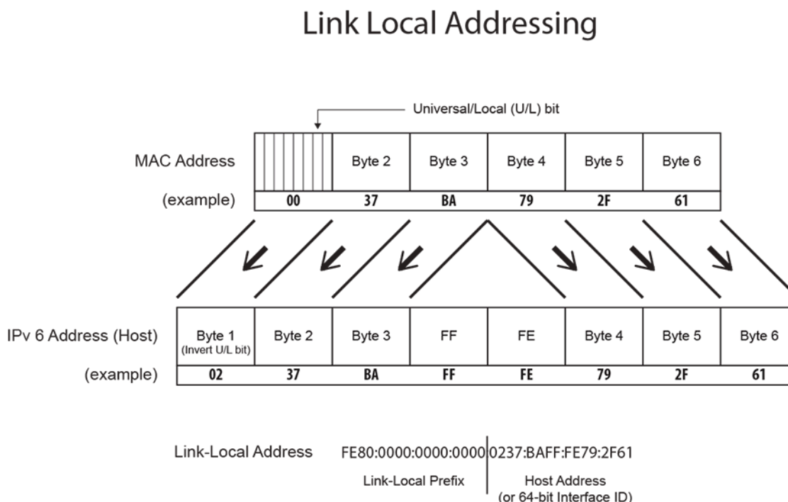
Figure 28: Link Local Address Derivation
