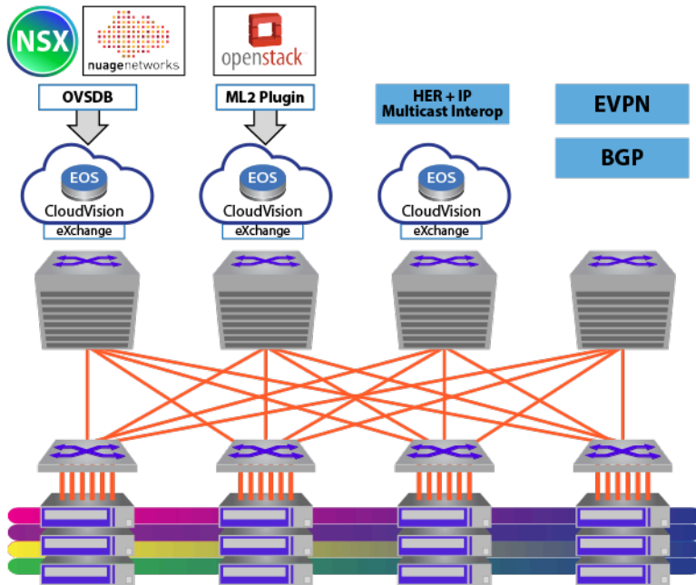
Figure 69: Different VXLAN Control Planes
