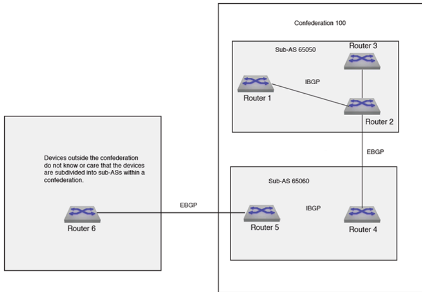
Figure 56: BGP Confederation Example
